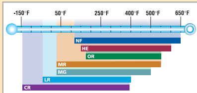
Temperature chart for selecting Paratherm brands.
